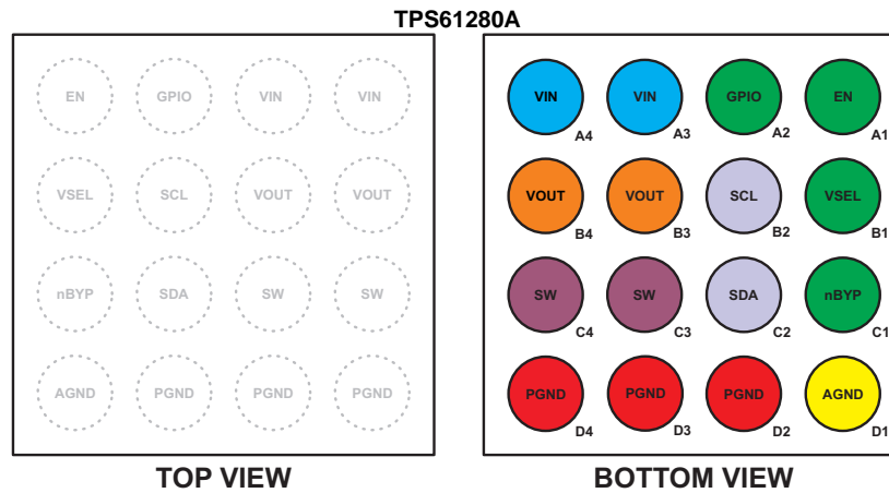
Pin Functions - TPS61280A
