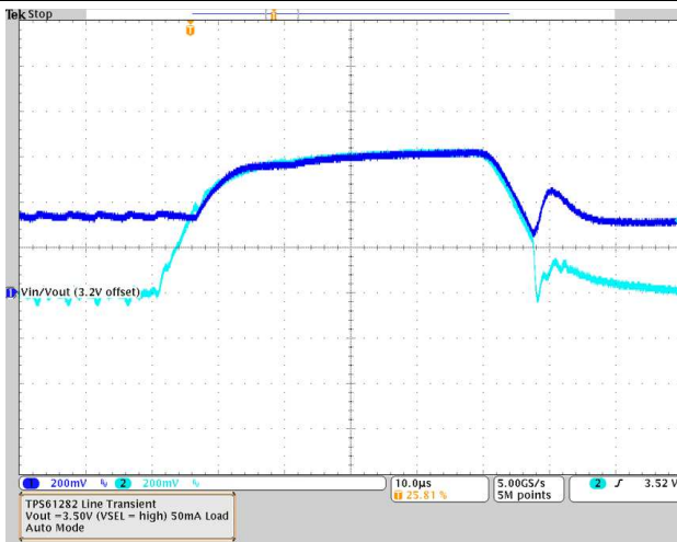
Figure 43. TPS61281A Forced Pass-Through to Boost Mode Transition
