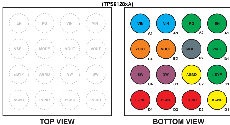
Pin Functions - TPS6128xA
